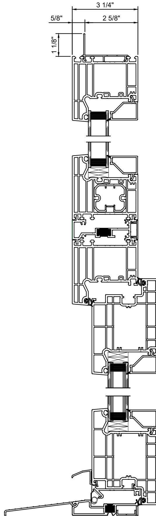
In-Swing Door w/ Transom
